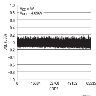
Differential Nonlinearity (LTC2600)
